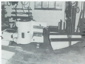
RADIAL DRILL ARMS - BROKEN IN TWO WHILE UNLOADING FROM TRUCK
